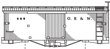
HOn3-31 Ohio River & Western Box Car
