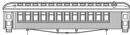
HOn3-25 D&RGW Closed Vestibule Coach
