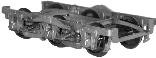
O-835- $39.50 (Plastic Kit) Six Wheel Pullman Trucks with Early Style Pedestals 10' 6" Wheelbase, 36" Wheels
