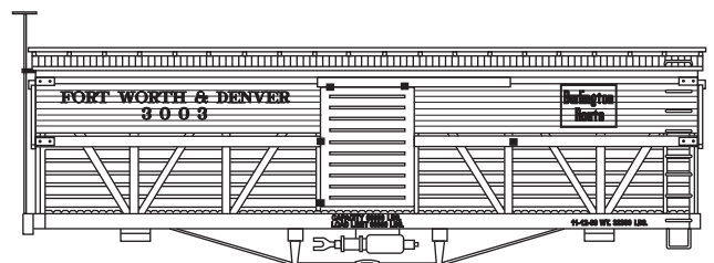
HO-53 Fort Worth and Denver Stock Car
