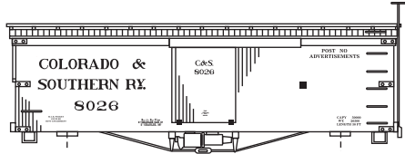
HOn3-111 C&S St. Charles Design Box Car
