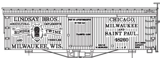
HO-56 Lindsay Bros. Box Car
