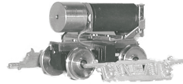
The Power Truck For HO Trolley and Traction Models. 5'7" Wheelbase, 36" wheels. Fully Self Contained, DCC Ready HO-810 Power Truck Only ..... $64.00 HO-811 Power Truck with Trailing Truck ..... $74.00
